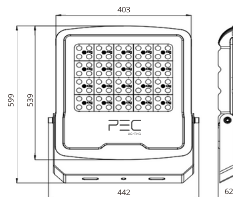
LED Floodlight Stadium 400W / 6000 K / 48000 lm
