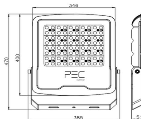
LED Floodlight Stadium 240W / 6000 K / 28800 lm
